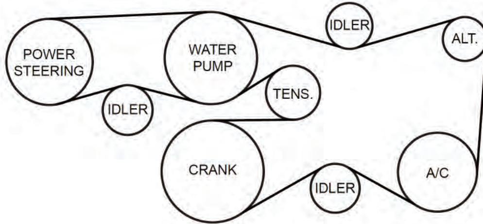
2010-2022 4RUNNER OEM BELT ROUTING
