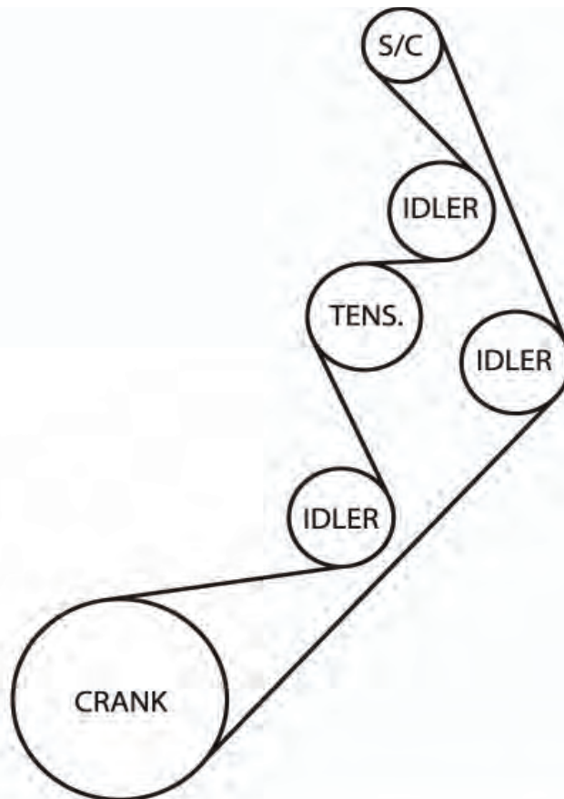
2010-2022 4RUNNER SUPERCHARGER BELT ROUTING
